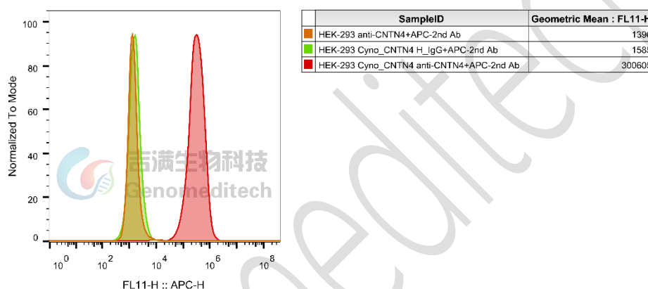
Figure 1 | Cynomolgus_CNTN4 HEK-293 Cell Line (Cat. GM-C42923) was determined by flow cytometry using Anti-CNTN4 hIgG4 Antibody(hAb-1) (Cat. GM-88283AB).
